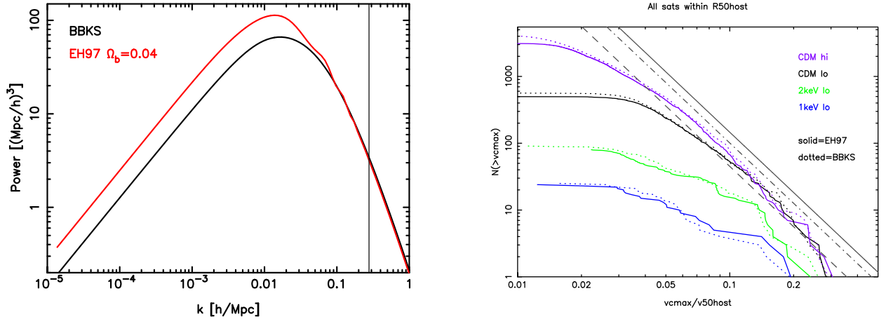
FIG. 11. Left Comparison of CDM power spectra calculated from the fitting formula of BBKS and Eisenstein & Hu (EH97). On scales k > 0.1 h/\text{Mpc} ( < 14 Mpc) the power spectra are nearly identical. The vertical line is the diameter of a spherical region with density \Omega_m \rho_c enclosing a Milky Way-sized mass 2 \times 10^{12} M_\odot ( \sim 5 Mpc). This scale is well within the range where the power spectra are nearly equal. Right Mass function comparison for set B simulations using fitting formula for CDM transfer function from BBKS ( dotted ) and Eisenstein & Hu ( solid ). The results are in good agreement
