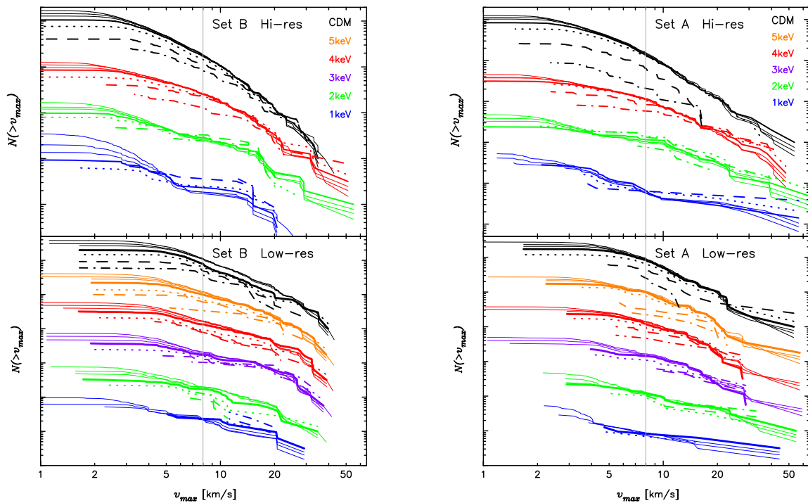
FIG. 8. (Left). Normalized mass functions for set B high (top) and low (bottom) resolution simulations. Thin solid lines are distances of 400, 300, and 250 kpc. Thick solid line is 200 kpc, dotted line is 150 kpc, dashed line is 100 kpc, dot-dashed line is 75 kpc. The WDM cosmologies have been shifted down vertically for clarity. The value \alpha = 0.55 was set by the high resolution simulation and provides good normalization for the low resolution as well but the effects of incompleteness become apparent at much larger radii (150 – 200 kpc compared to 75 – 100 kpc for high res). (Right). Same as the left panel, but for the set A high (top) and low (bottom) resolution simulations. The value \alpha = 0.55 also provides good normalization for this set of halos.
