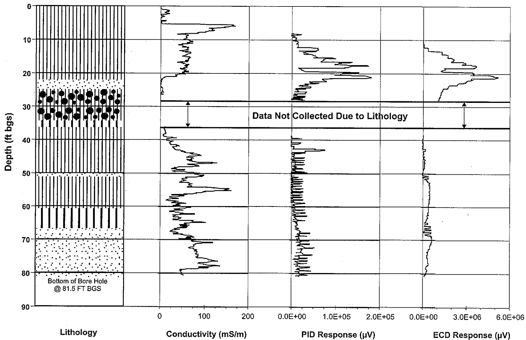
Figure 2.4 VERTICAL PROFILE OF VOCs AND SOIL CONDUCTIVITY PRODUCED BY MIPS
