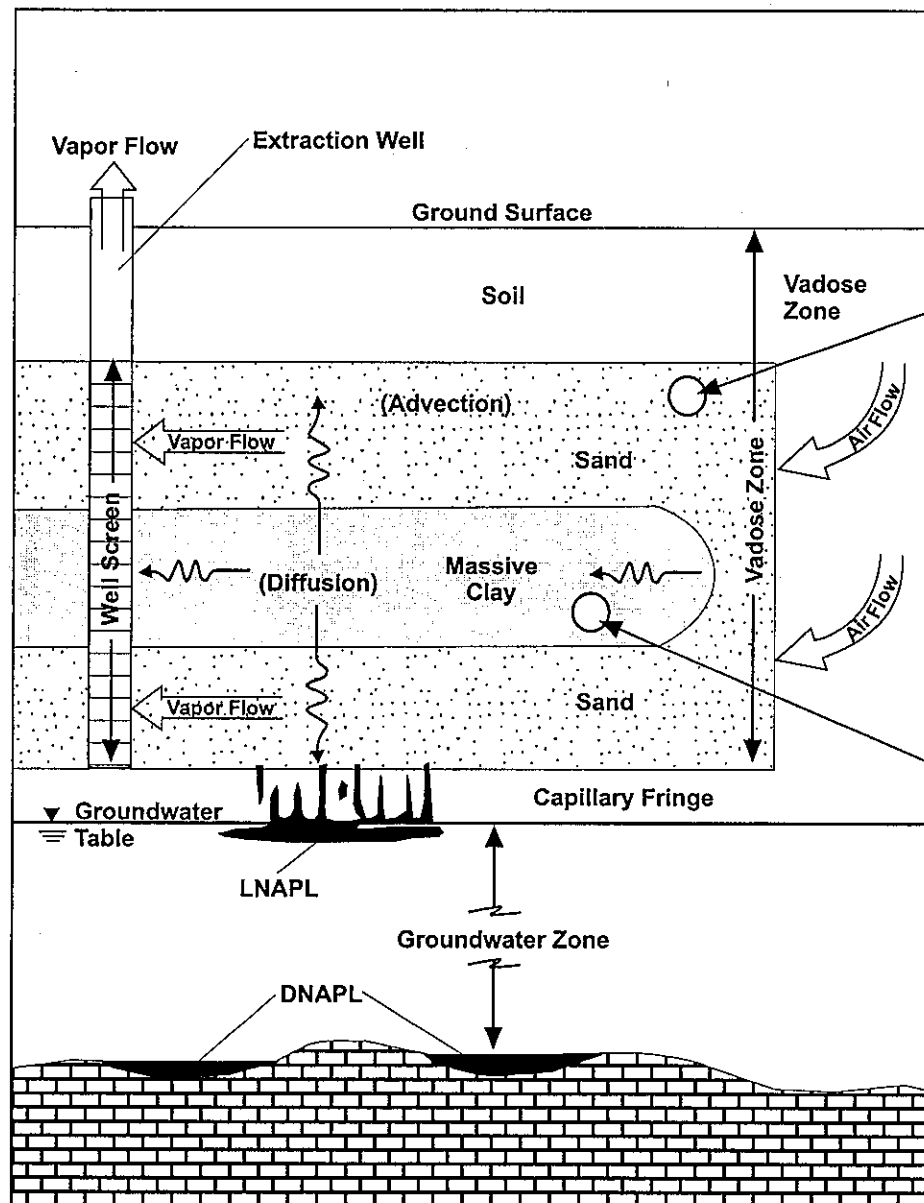
Figure 1.2 VOLATILE ORGANIC FATE AND TRANSPORT PROCESSES
