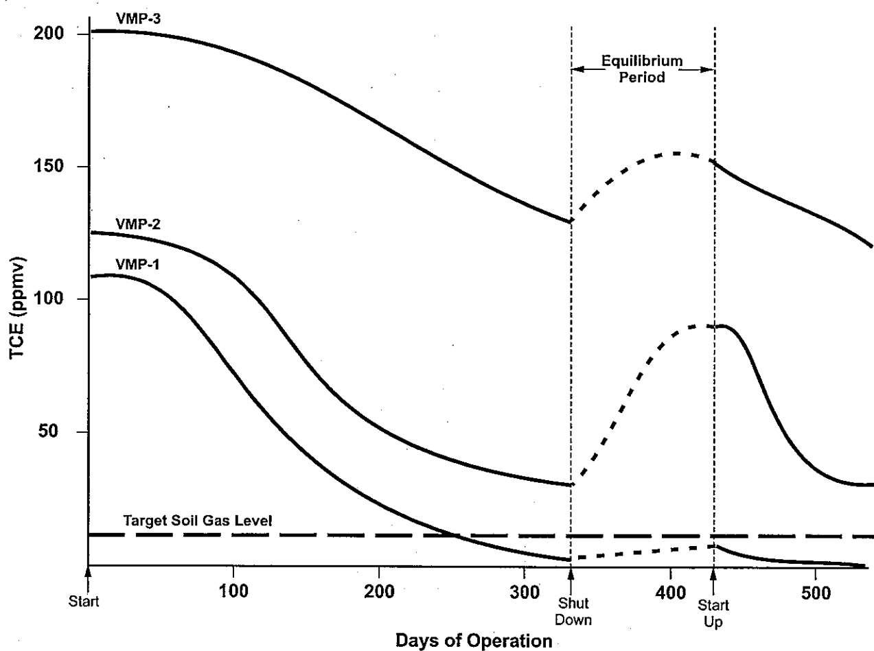
Figure 4.4 RESULTS OF EQUILIBRIUM / REBOUND TEST
