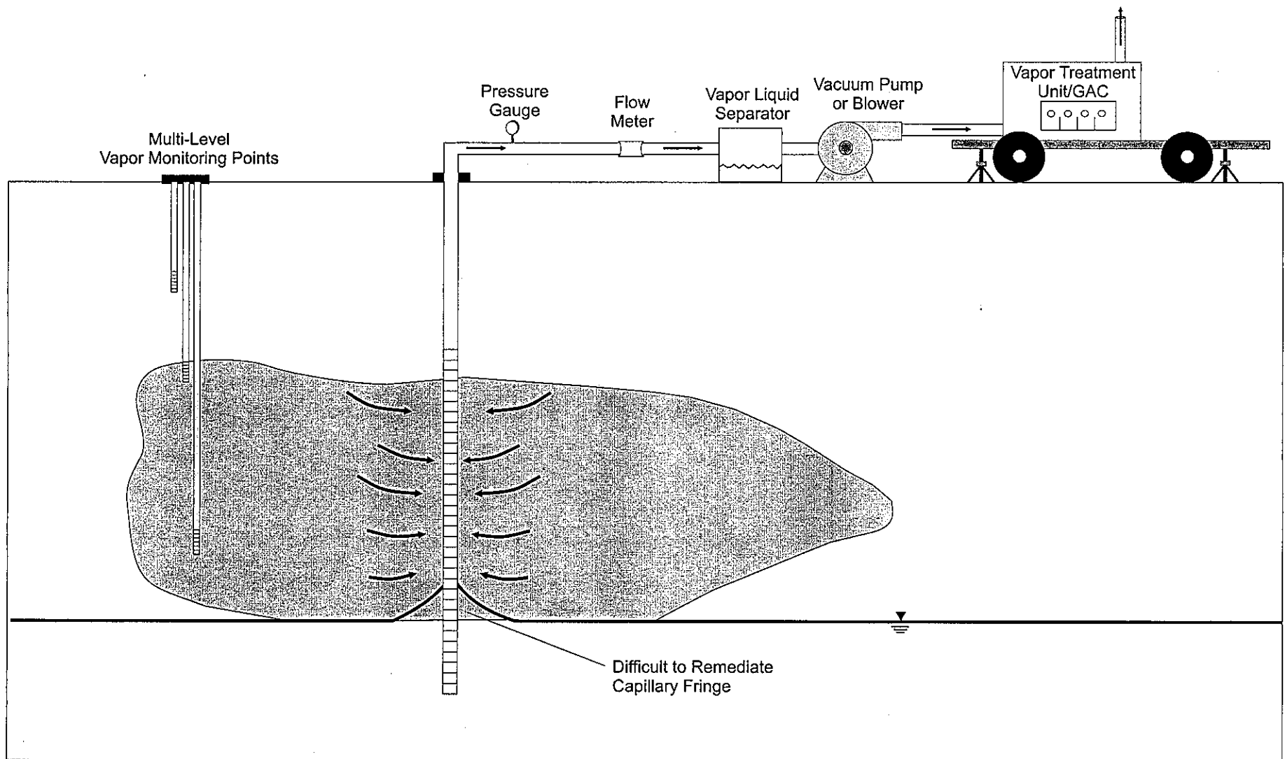
Figure 1.1 BASIC IN-SITU SOIL VAPOR EXTRACTION SYSTEM
