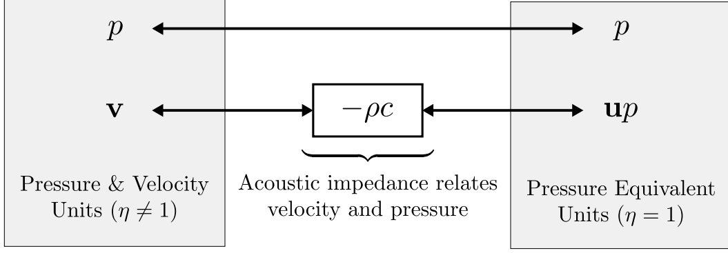
Figure 1.7.1: Vector-sensor measurements, scaled to common units
