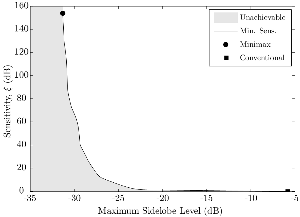
Figure 4.3.8: Minimum sensitivity versus maximum sidelobe level
