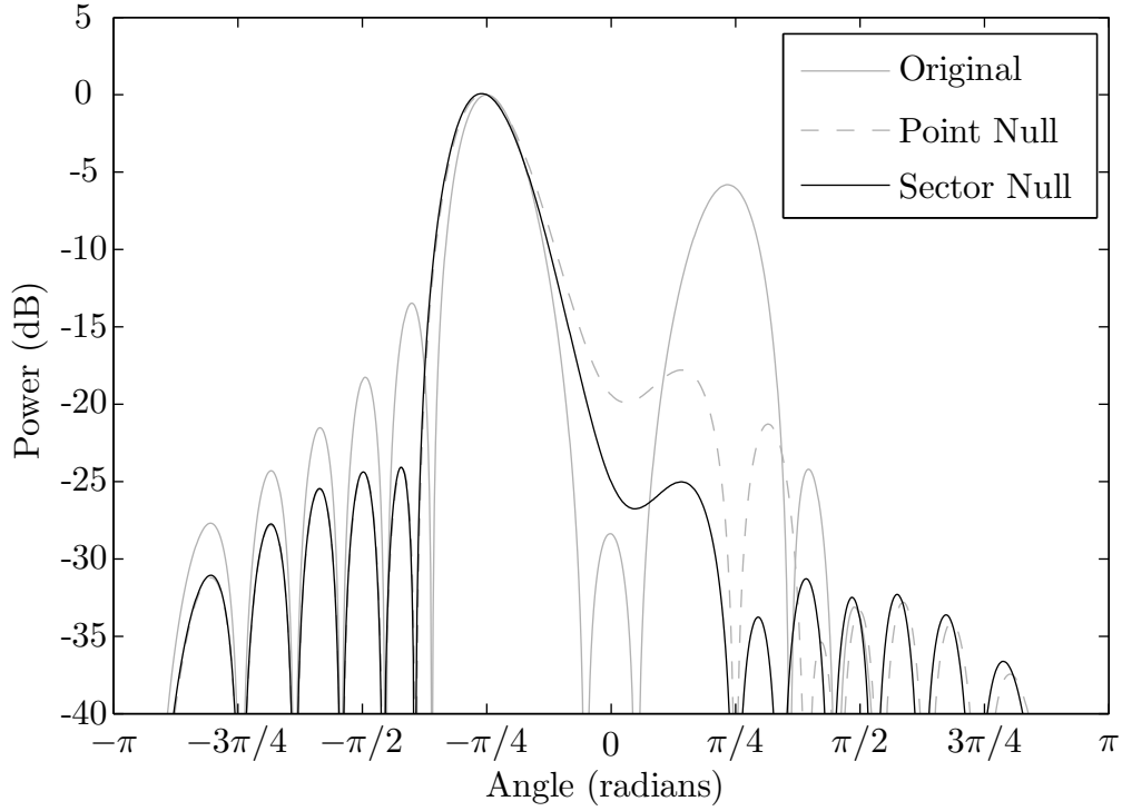
Figure 4.2.1: Comparison of tapered point and sector null beampatterns
