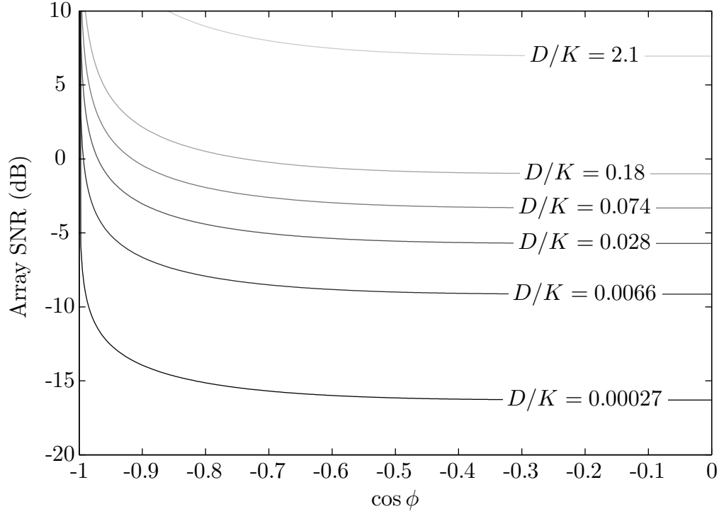
Figure 3.1.4: Divergence contours: f = \frac{5}{7}f_d , N = 10
