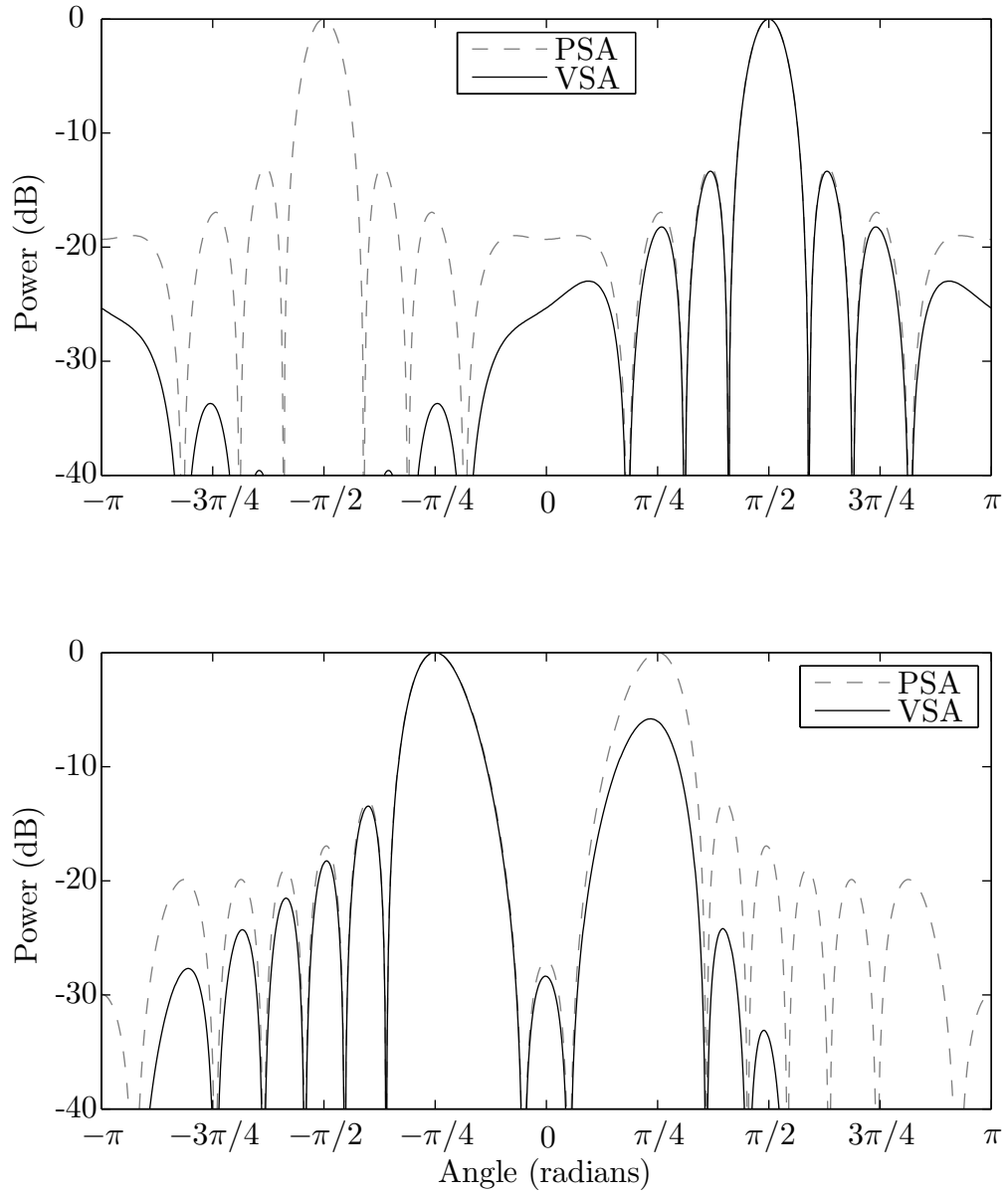
Figure 1.3.2: Example VSA and PSA response patterns
