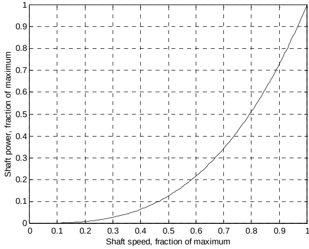
Figure 3: Normalized propulsion power
