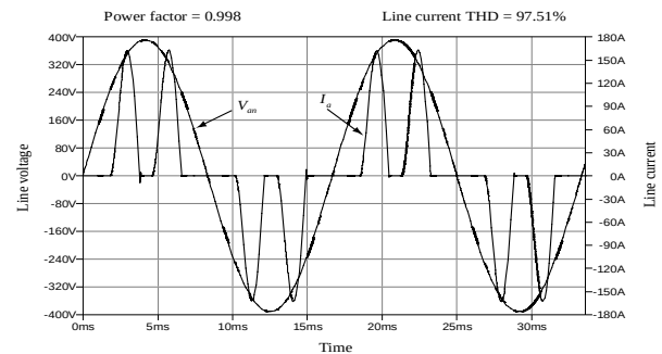
Figure 10: Simulated line waveforms
