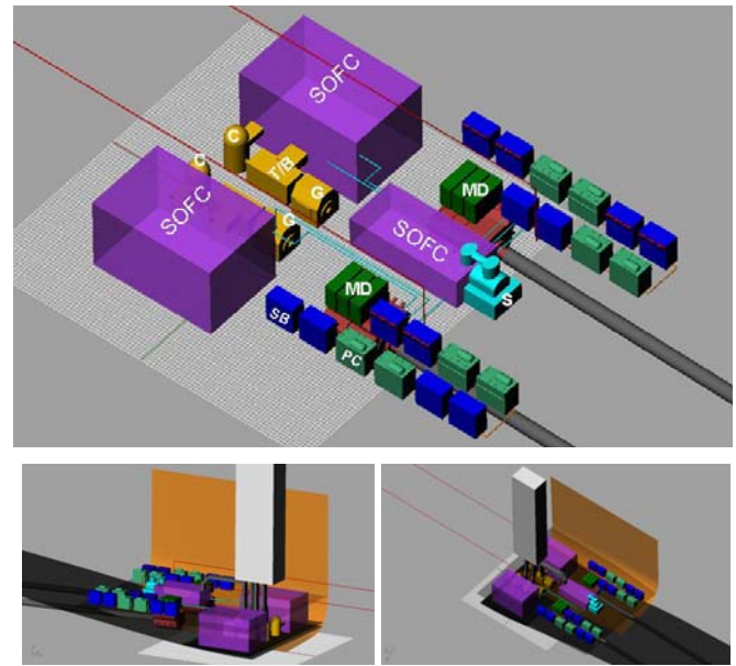
Figure 14: Machinery arrangement of configuration A.
