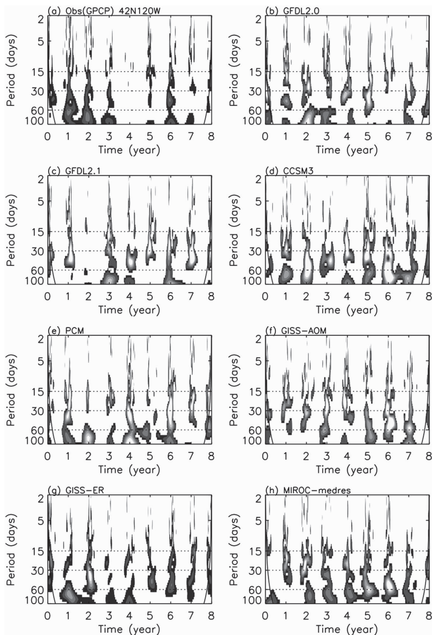
FIG. 6. Wavelet spectrum of precipitation averaged between 40°–45°N, 125°–115°W.
