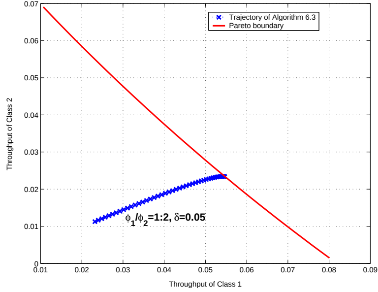
Figure 6.7: The trajectory of Algorithm 6.3.
