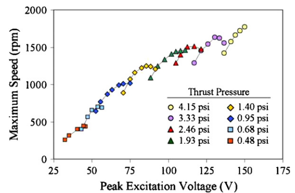
Figure 8. Maximum achievable speed as a function of the peak sinusoidal voltage for various thrust pressures.
