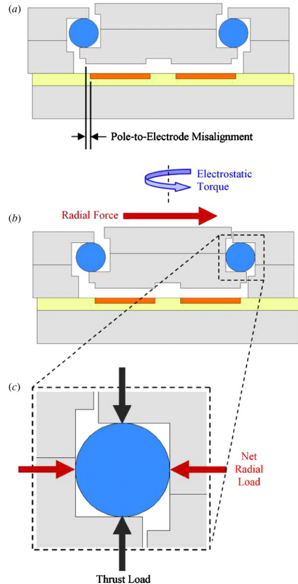
Figure 11. Schematic of the misaligned assembly showing (a) the rotor-to-stator layer misalignment, leading to (b) an electrostatic radial force during actuation, which results in (c) a net radial load supported by the microballs.
