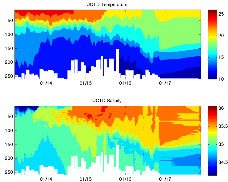
Figure 5-5. Upper: Temperature ( ^{\circ}\text{C} ) measured by UCTD. Lower: Salinity (psu) derived from measured pressure, temperature and conductivity.
