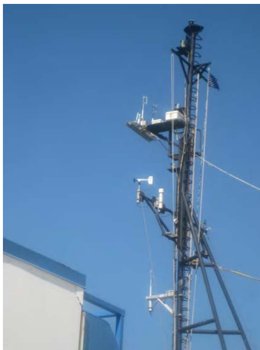
Figure 5-18. Turbulence Flux system setup on the jack staff of the NOAA Ship Ronald H. Brown . WHOI turbulent anemometer is at lowest level.
