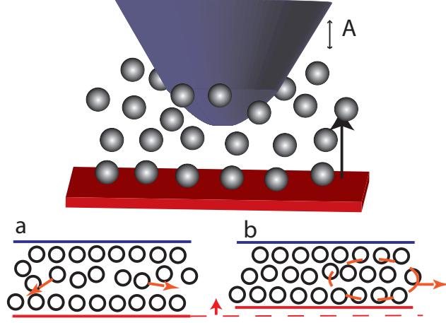
FIG. 1. (color online) Schematic showing the mica substrate approach the AFM tip, while water molecules are confined in the gap. The AFM tip is oscillated at an amplitude smaller than the molecular size. a. The confined water layer is between three and four molecular layers thick, and does not exhibit ordered layers. Therefore, molecules have sufficient space to easily diffuse. (tip represented by top, blue line) b. Water layer is further compressed until the gap corresponds to three molecular layers. Molecules are ordered in the vertical direction into layers, and cannot easily move individually. Squeeze-out of a layer requires collective motion of many molecules.
