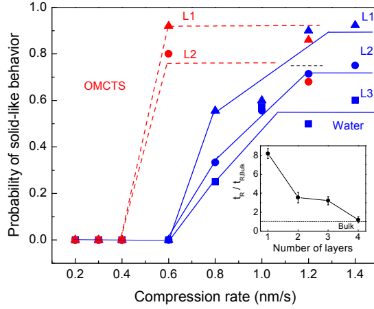
FIG. 3. (color online) Probability that layers show solid-like mechanical behavior. Blue: Water with 1 (L1) to 3 (L3) confined layers (L3). Red: OMCTS with 1 (L1) to 2 (L2) confined layers. Lines guide the eye and do not imply any functional relationship. Inset: Mechanical relaxation time versus number of confined layers in water, averaged for all rates above 8 Å/s. Relaxation time strongly depends on layer number as shown, but is independent of squeeze rate as long as dynamical solidification is observed.
