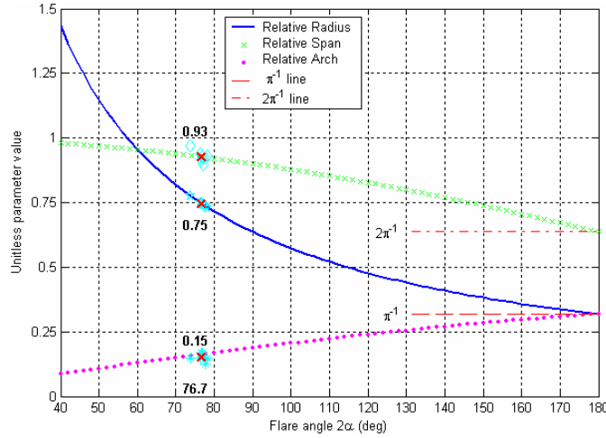
Figure 5. Dependences of relative front-view geometry parameters on the flare angle.
