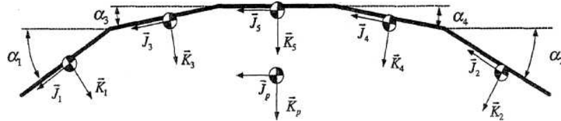
Figure 1. Parafoil canopy geometry used by Slegers and Costello. 64
