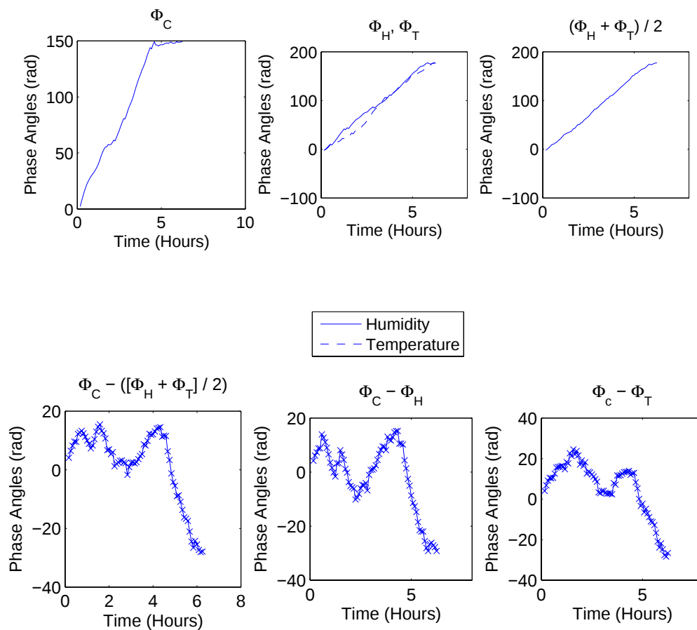
Figure 8. March 28, 2004 morning. Humidity dominates.
