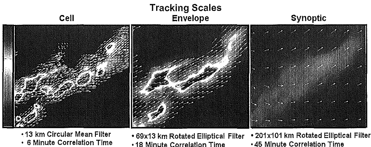
Figure 2a: Three scales used to create raw motion vectors from smallest to largest: cell, envelope, and synoptic. Motion vectors are shown in white, the background is a spatially filtered interest image. VIL is passed through the filters, then correlated with previous images to calculate the motion vectors.
