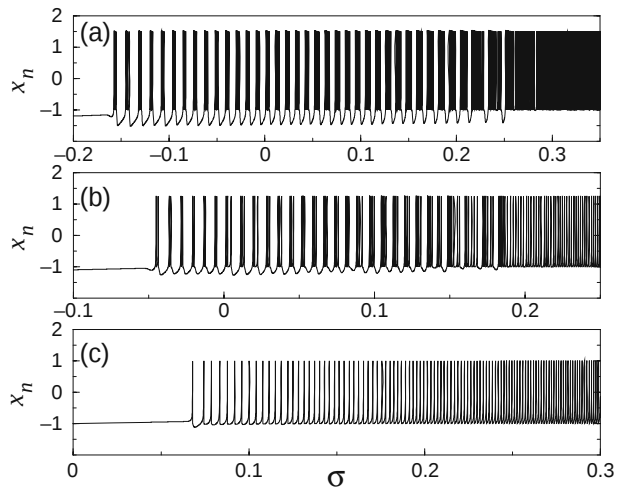
Fig. 2 Restructuring of oscillation in map (4) with a \alpha=5.0 , b \alpha=4.5 , and c \alpha=4.0 , as the value of \sigma increases with the constant slew rate \Delta\sigma = 0.00005 per iteration
