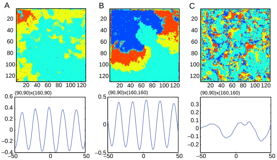
Fig. 15 Oscillations in two-dimensional network model of 256 \times 256 PY neurons and 128 \times 128 INs. Snapshots of activity in inhibitory, IN, population (top) and cross correlation of local FPs (average activity of 100 \times 100 PY neurons) between two remote spatial areas (bottom) are shown. a Nearly global synchronization—phase locking with zero phase shift, g_{PY-IN}=0.002 , g_{IN-PY}=0.0007 . b Local synchronization mediated by two rotation spiral waves, g_{PY-IN}=0.0015 , g_{IN-PY}=0.0007 . c Asynchronous state, g_{PY-IN}=0.002 , g_{IN-PY}=0.0015 . In top panels, red, depolarizing (spikes), and blue, hyperpolarizing potentials
