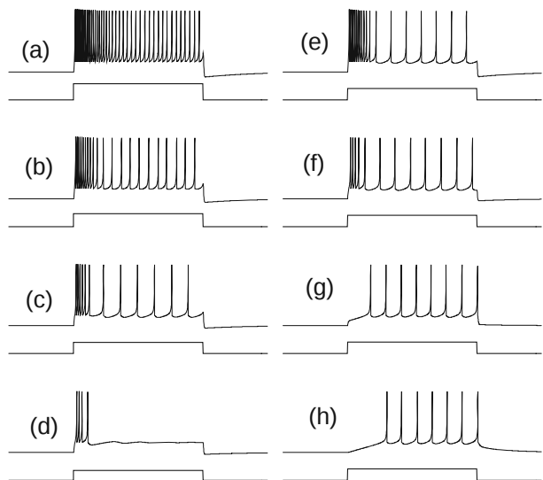
Fig. 3 Waveforms of x_n for the responses of map (4) to a rectangular pulse of amplitude I_a and duration 1,000 iterations computed for different pulse amplitudes ( left ) and the input balance parameter \beta^e ( right ). The shapes of the pulse are shown below the traces of x_n . The parameter values are \alpha = 4.0 , \sigma = -0.4 , \sigma^e = 1.0 , and a - I_a = 0.630 , \beta^e = 0.224 ; b - I_a = 0.517 , \beta^e = 0.224 ; c - I_a = 0.439 , \beta^e = 0.224 ; d - I_a = 0.394 , \beta^e = 0.224 ; e - \beta^e = 0.3 , I_a = 0.45 ; f - \beta^e = 0.2 , I_a = 0.45 ; g - \beta^e = 0.1 , I_a = 0.45 ; h - \beta^e = 0.0 , I_a = 0.45
