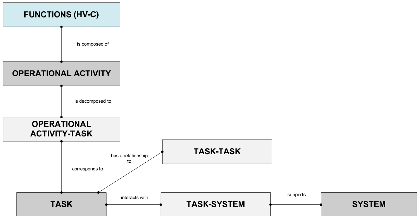
Figure C.3. Data Model for HV-C Tasks
