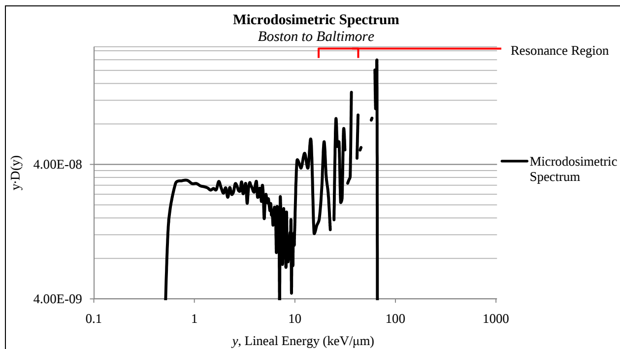
Figure VIII.17 – Microdosimetric Spectrum for Flight from BOS to BWI
