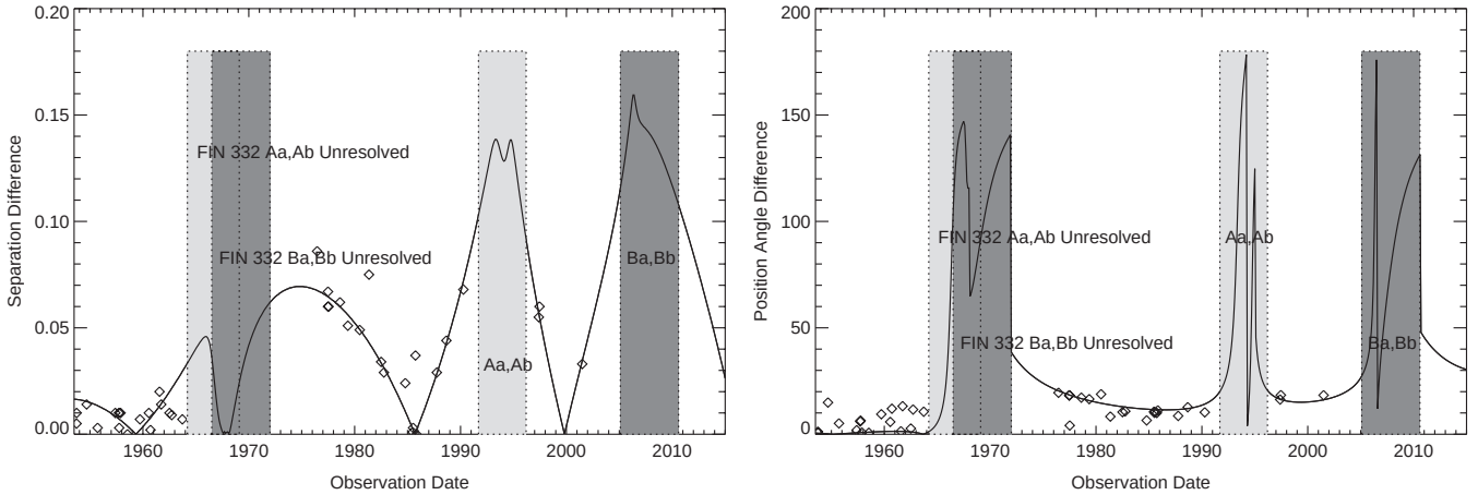
Figure 2. Difference in separation and P.A. between FIN 332 Aa, Ab and Ba, Bb. The solid curve indicates the predicted difference based on the orbits of Section 5.1. The diamonds represent the differences between measures of Aa, Ab and Ba, Bb when they were made at the same time by the same observer. The lighter shaded areas from 1964.2 to 1969.1 and 1991.7 to 1996.2 are dates when Aa, Ab is predicted to be closer than 0''.05 . The darker shaded areas from 1966.5 to 1972.0 and 2005.1 to 2010.6 indicate the range of dates when the orbit predicts Ba, Bb to be closer than 0''.05 .
