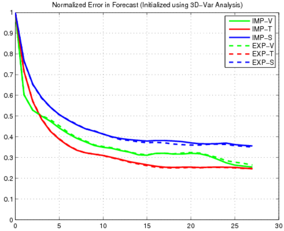
Figure 7: Relative forecast error in T (red), S (blue), and total v (green) for 3DV-IMP (solid) and 3DV-EXP (dashed). Relative error is normalized by error in each field at day 1. Error is calculated as in (8).
