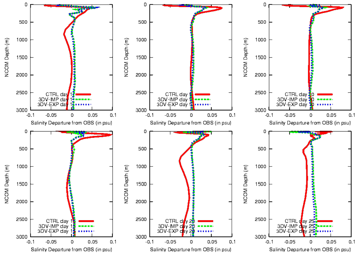
Figure 6: Same as in fig. 5, but for salinity.
