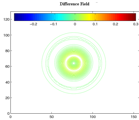
Figure 2: Example correlation function centered at 78x65 on arbitrary grid; center value is 1.0 for (a) the explicit solver and (b) the implicit solver; (c) displays the difference field explicit minus implicit. Grid resolution and correlation length scale are fixed at 6.0 \times 10^3 m and 6.0 \times 10^4 m, respectively.
