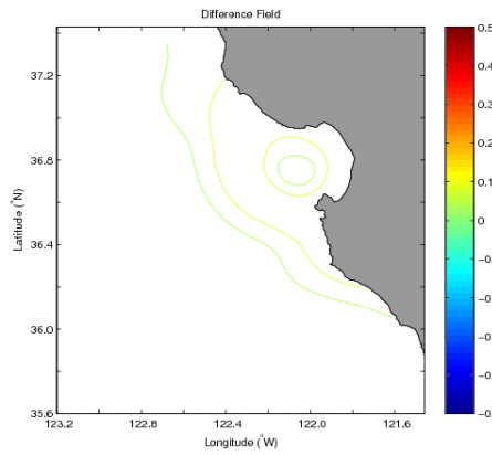
Figure 3: Anisotropic correlation function (with length scale modification) near the coast of Monterey Bay, California, U.S. A. using the (a) explicit and (b) implicit solver; (c) shows the difference field explicit minus implicit; (d) shows the bathymetry.
