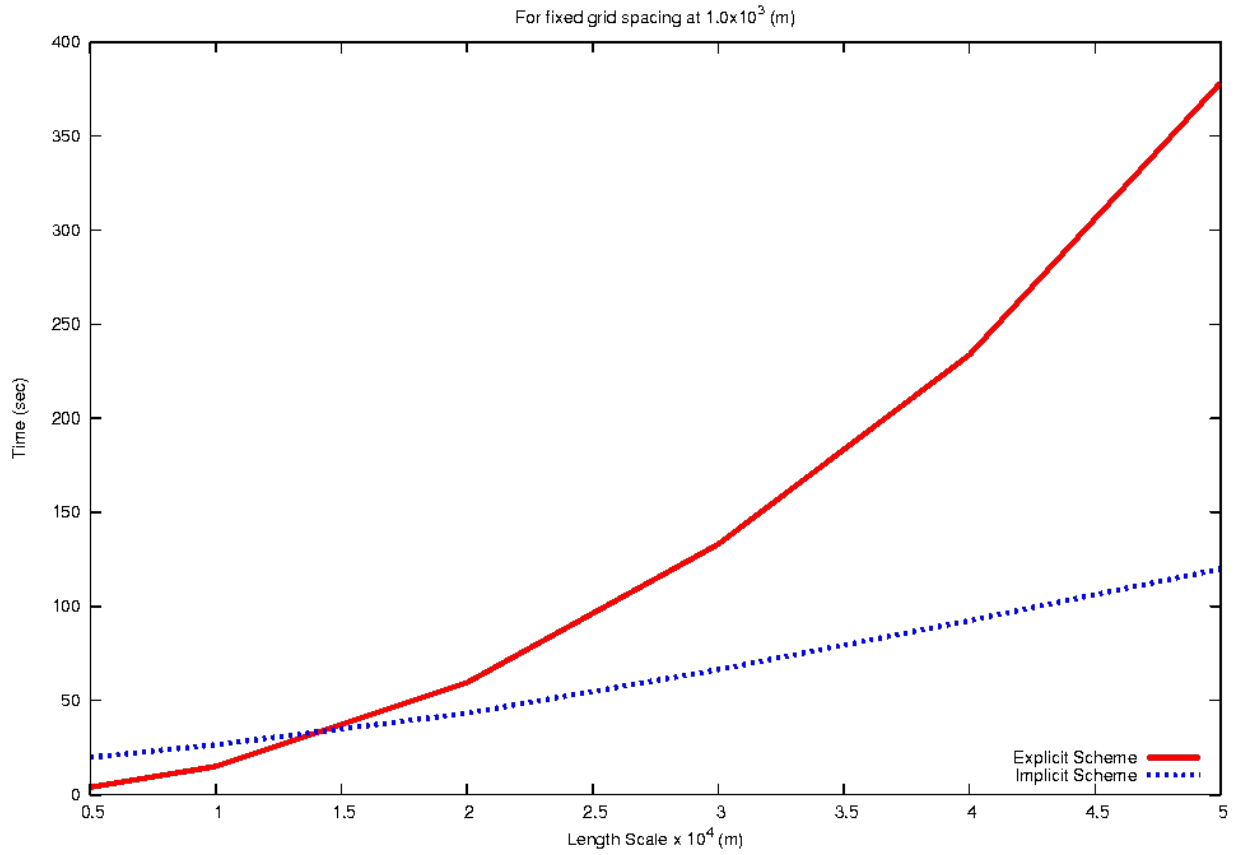
Figure 1: CPU time to run diffusion-based correlation operator for a fixed grid resolution and varying correlation length scales. Implicit solver in dashed blue, explicit in solid red; y-axis is CPU time (in seconds) and x-axis is correlation length scale (in 10^4 m).
