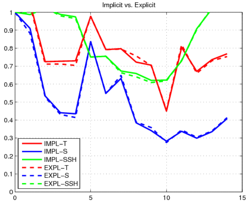
Figure 10: Relative forecast error in T (red), S (blue) and SSH (green) for IMPL model run (solid) and EXPL model run (dashed). Relative error is normalized by error in each field at day 1. Error is calculated as in (8).
