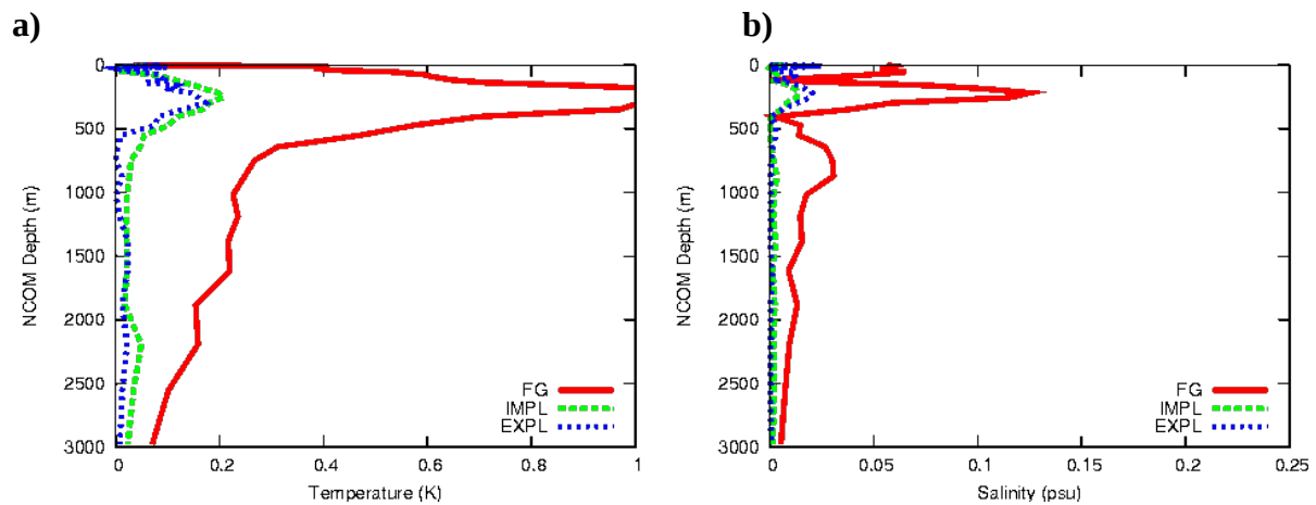
Figure 9: Absolute difference between observation profile and first guess (FG) profile (red), analysis that used the implicit solution correlation operator (green), and analysis that used the explicit operator (blue). Left (a) is for temperature, panel (b) is for salinity. Comparison is valid at 0000 UTC 16 June, 2008.
