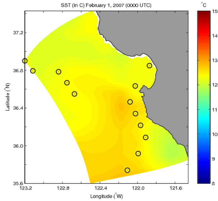
Figure 4: 13 T/S profile locations selected in NCOM domain for simulated ocean data assimilation experiment. Field shown is SST (in °C) for 1 February, 2007 at 0000 UTC.
