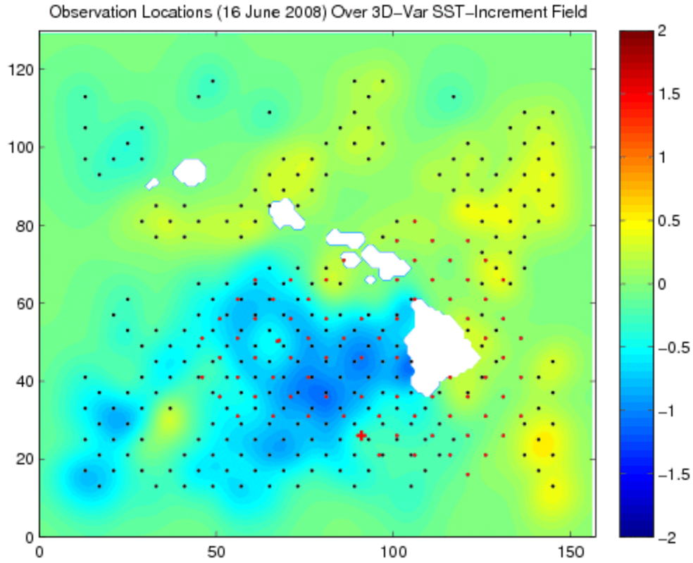
Figure 8: All temperature observation locations for 16 June, 2008 including surface observations (black dots) and profile observations (red dots) overlaid on 3D-Var surface temperature increments. Location of excluded profile used as independent observation indicated by red cross.
