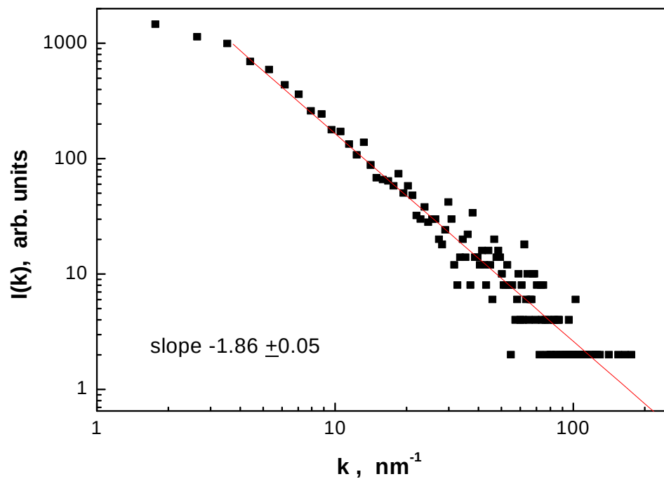
Figure 14. Surface roughness power spectrum for the 480 nm thick silicon film exfoliated under annealing temperature of 400° C from the boron free silicon wafer. Scanning window is 6.3×6.3 \mu\text{m}^2 .
