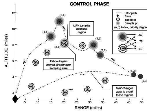
Figure 2: One UAV trajectory as determined by the real-time control algorithm.
