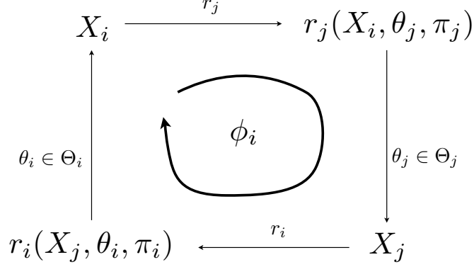
Figure 2.1. \phi_i mapping
