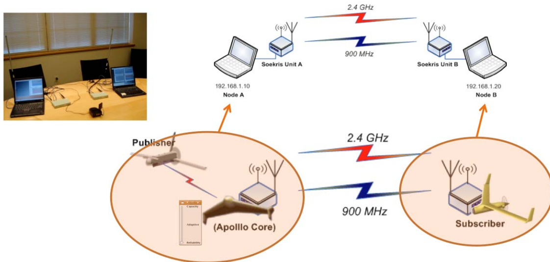
Figure 10. Experimental Setup for Dual-Link Management Controller
