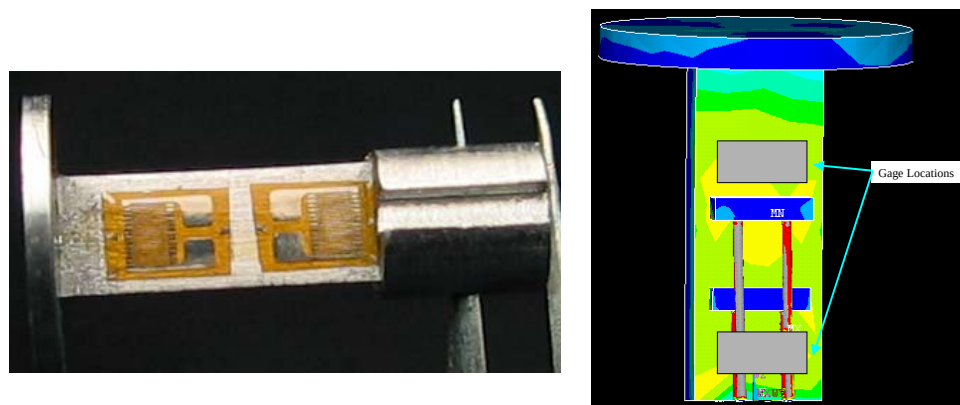
Fig. 29. Strain gage application (right). Compressive side strain distribution from a 2000 Pa shear load (right). FEM from ANSYS®.
