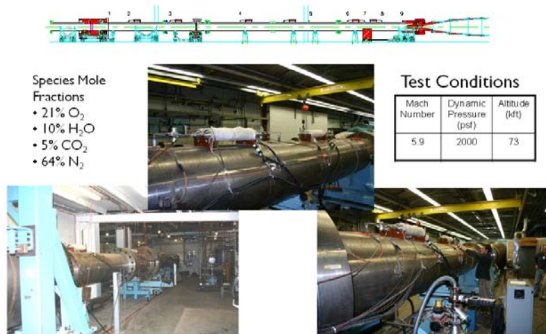
Fig. 42. System to add vitants to tunnel reservoir
