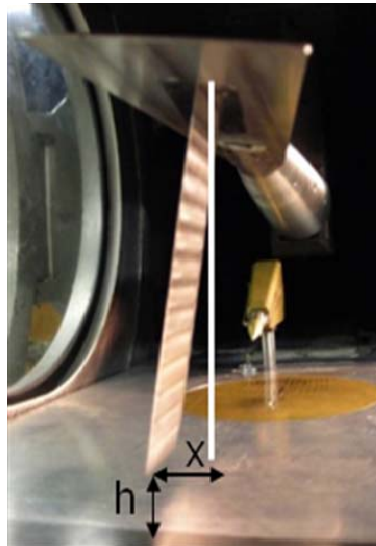
Fig. 26. Photograph of the vortex generator and sampling probe in the VT supersonic wind tunnel. The location of the vortex is defined by (x, h) .
