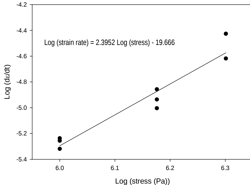
Figure 1 Strain rate vs. stress for conventional creep measurements, Nb at 1,985 °C under 1.0, 1.5, and 2.0 MPa.
