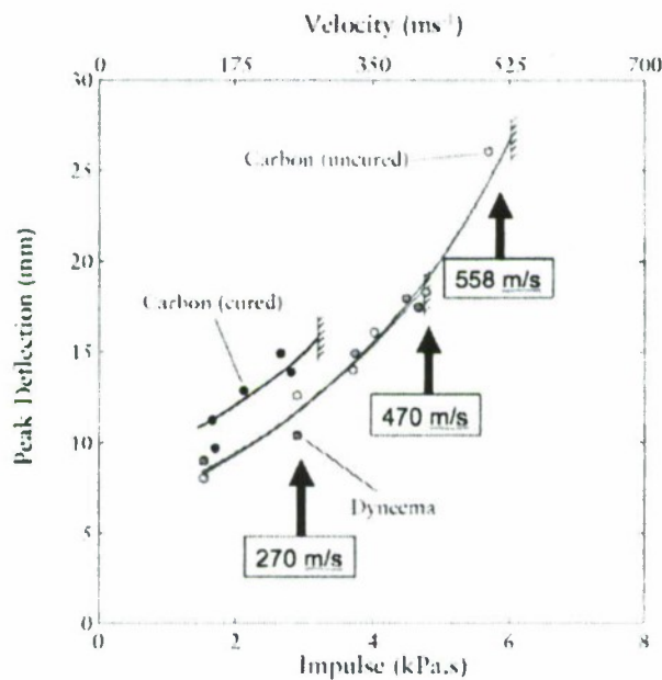
Figure 12: The relative blast performance of Dyneema® and 0/90 CFRP panels of equal areal density.
