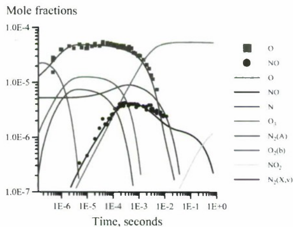
Fig. 8: Experimental O atom and NO concentrations (symbols) and species concentrations predicted by Model II (“N 2 (v)” model, lines) after a single-pulse discharge in air. P= 60 torr.
