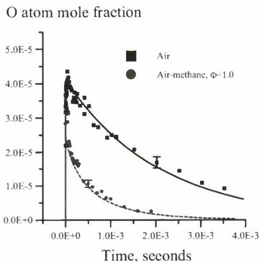
Figure 2. Oxygen atom mole fraction vs. time after a single high-voltage pulse in air and in a methane-air mixture at P=60 torr and \Phi=1.0 .
