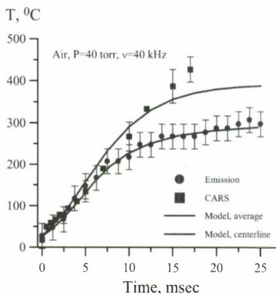
Figure 4: Comparison of experimental spatially averaged (emission) and centerline (CARS) temperatures in a repetitively pulsed nanosecond discharge in air at P=40 torr with plasma chemistry model prediction.
