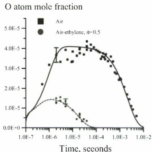
Figure 3. Oxygen atom mole fraction vs. time after a single high-voltage pulse in air and in an ethylene-air mixture at P=60 torr and \Phi=0.5 .
