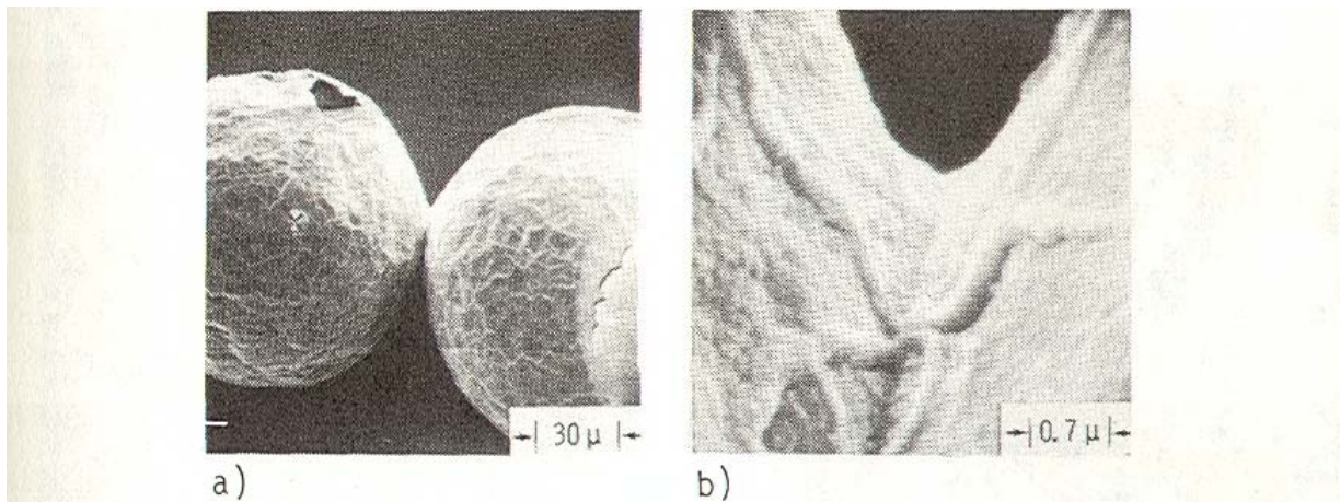
Fig. 3 Cooled particles that have been heated to 1400^{\circ}\text{C} on a sapphire plate in an oxygen-containing atmosphere: a) cracked oxide shells evident; b) oxidation healing of cracks, including
