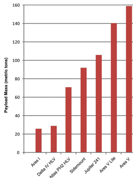
Figure 5.2-1. Approximate payload mass launched by various launch vehicles to a 28.5 degree inclination low-Earth orbit. Source: Review of U.S. Human Spaceflight Plans Committee
