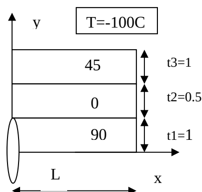
Figure 2.4 1/4 of the laminate repeating element with a crack in the central layer.
