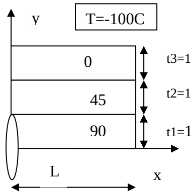
Figure 2.5 1/4 of the [0,45,90] s laminate repeating element with a crack in the central layer.
