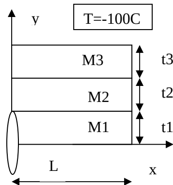
Figure 2.1 \frac{1}{4} of the laminate repeating element with a crack in the central layer.
