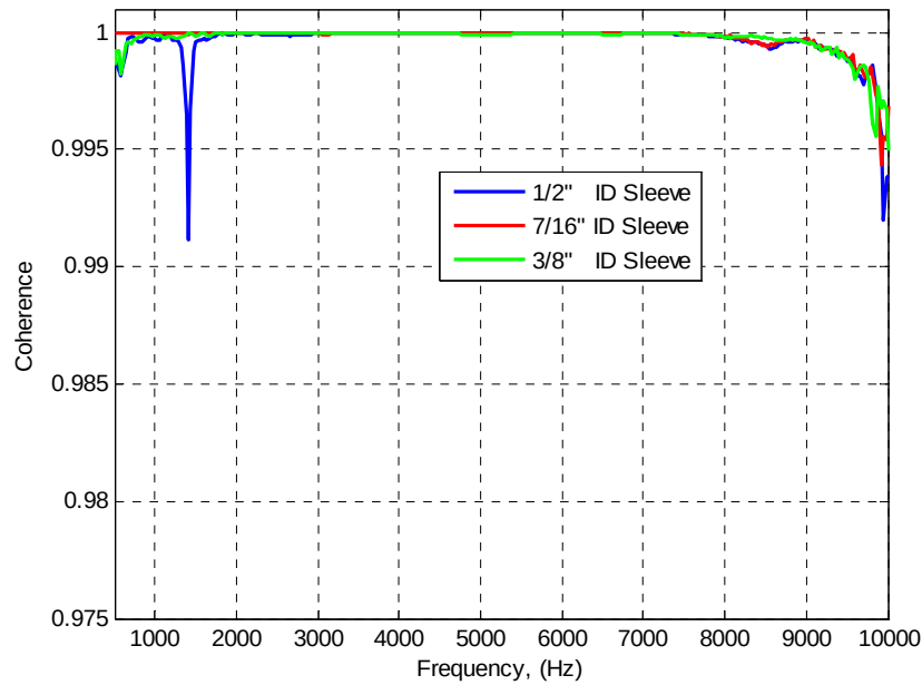
Figure 4.11 Coherence for all three shear preload cases.
