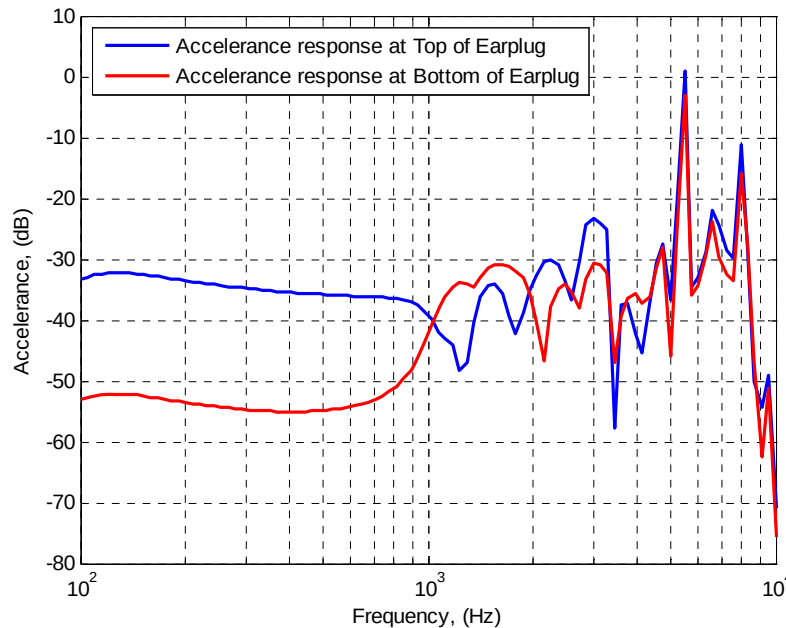
Figure 6.13 Comparing the accelerance of the top and bottom of the Ear foam earplug.
