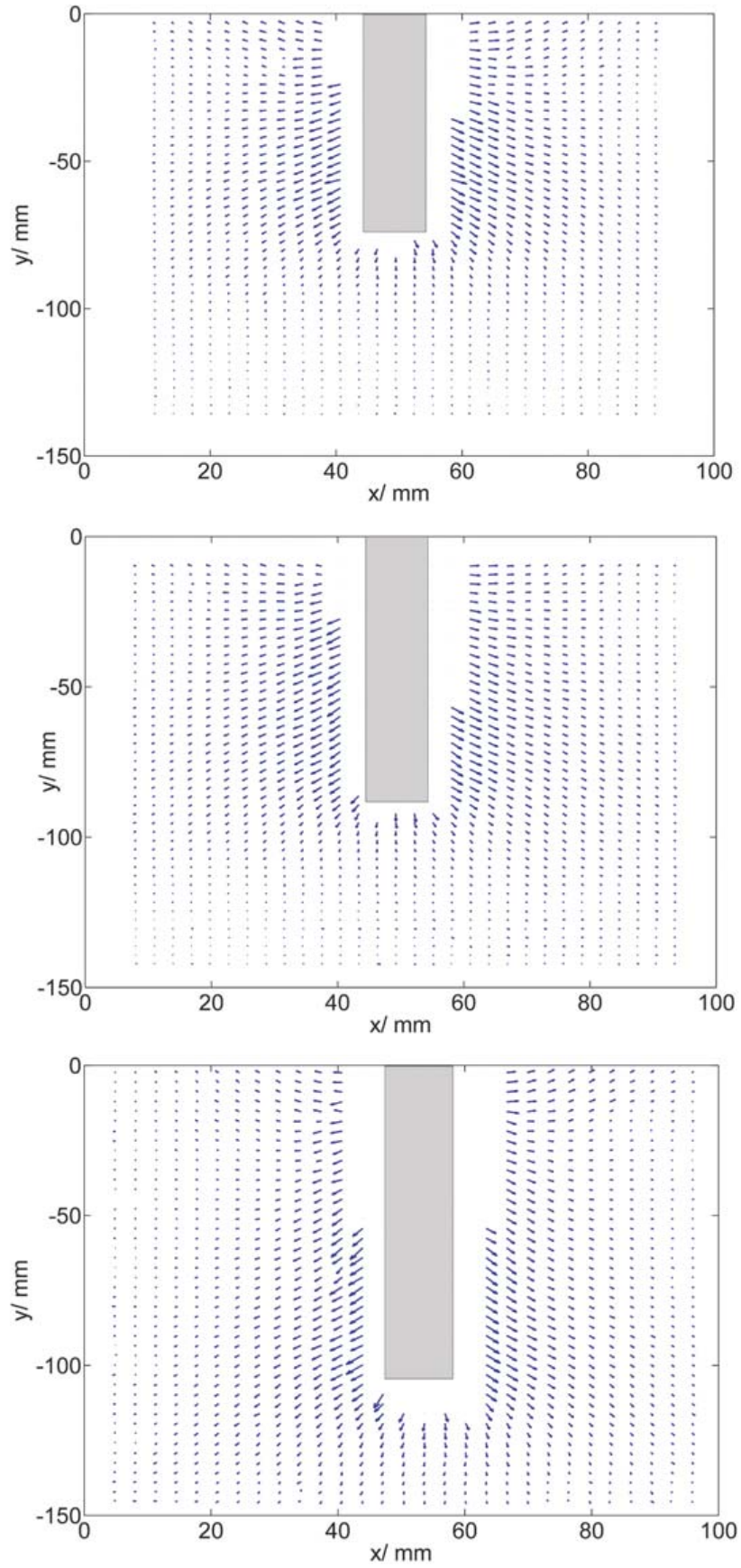
Figure 13. Scaled quiver plots showing penetration by a flat ended rod at 450, 550 and 750 \mu s after impact.
