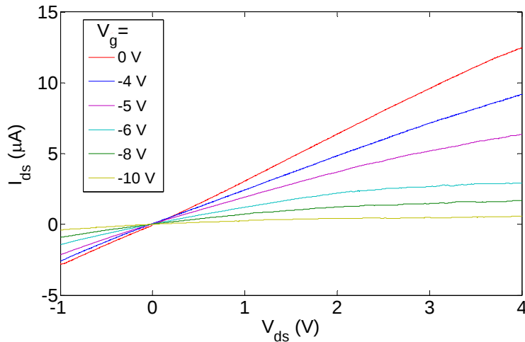
Figure 3 : Typical I_{ds} versus V_{ds} curves of 28 nm diameter and 1.6 µm length n-type SiNWs, The back-gate voltage for each curve is indicated.
