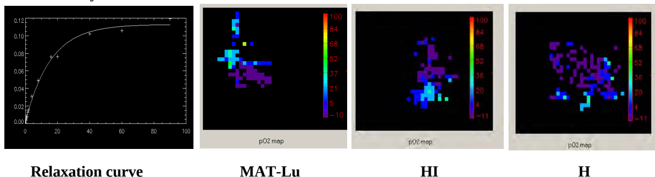
Figure 1. Oximetry in Dunning prostate tumors. Left A typical ^{19}F NMR T_1 relaxation curve for the signal intensity of the reporter molecule hexafluorobenzene from a single voxel within a tumor. The relaxation rate is directly proportional to pO_2 . Based on such curves, maps were generated for representative MAT-Lu, HI and H tumors growing on anesthetized rats breathing air with isoflurane anesthesia. Voxel dimension 1.25 mm in plane with 10 mm thickness.
