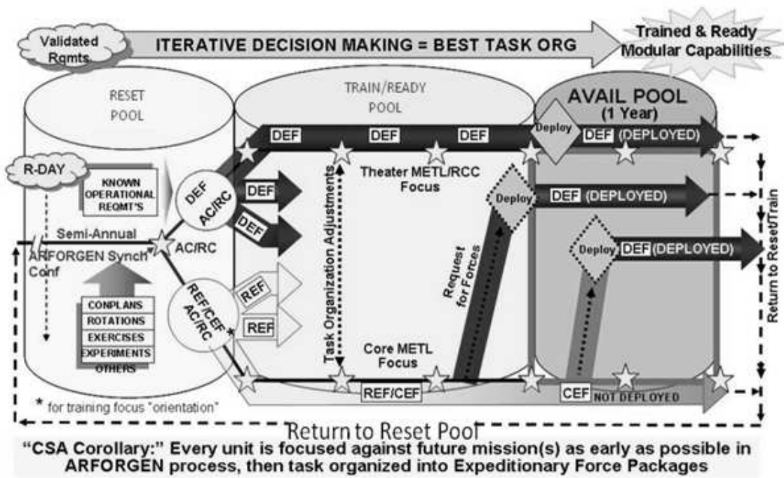
Figure 2. ARFORGEN Process
