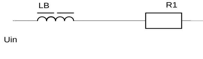
Fig.4. Equivalent circuit of the power supply with a ballast inductor coil.
