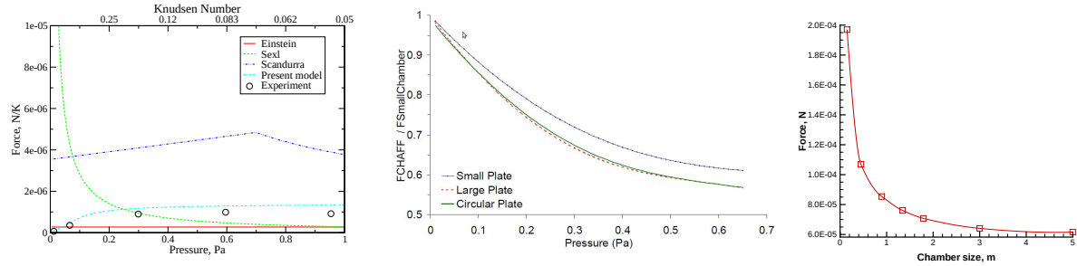
FIGURE 5. Left: analytic estimates of radiometric force in argon as compared to the data. Center: measured large chamber to small chamber force ratio for different vane geometries. Right: chamber size dependence of radiometric force modeled with DSMC.
