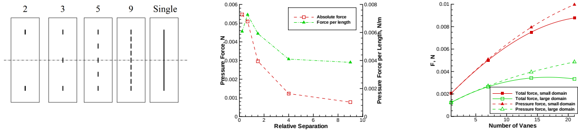
FIGURE 7. Left: multi-vane computational setup. Center: impact of vane separation on total force. Right: force increase in multi-vane geometries.
