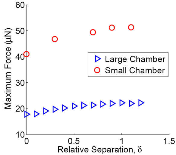
FIGURE 4. Maximum force as a function of separation for Large and Small Chamber Configurations.
