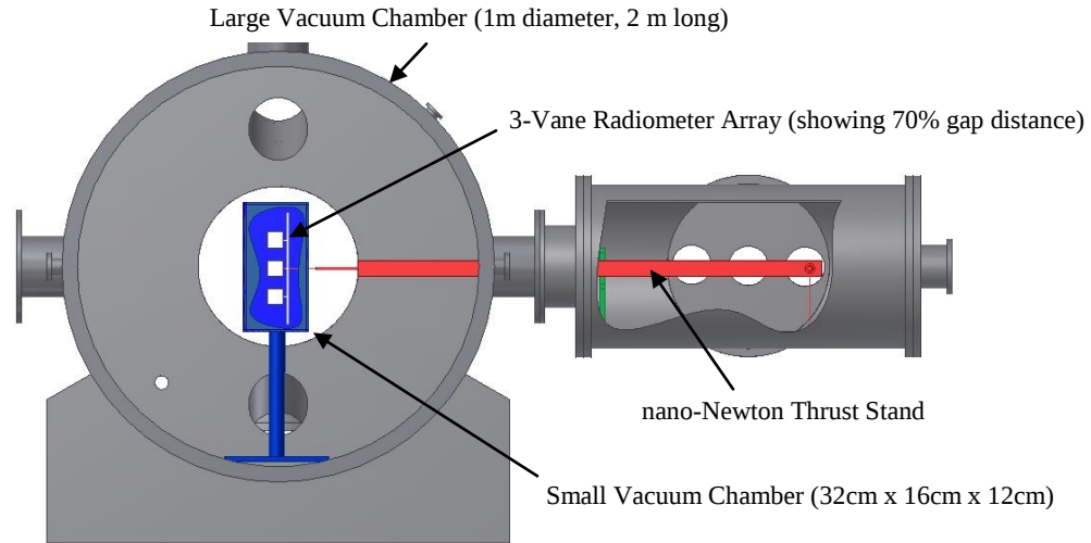
FIGURE 1. Radiometer Vane Array Experimental Set Up.
