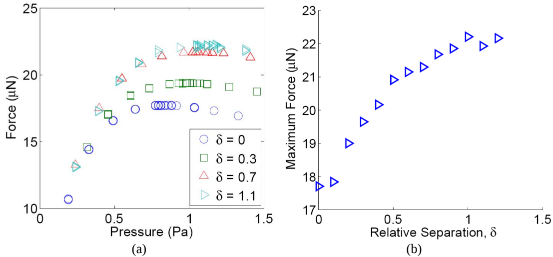
FIGURE 3. Experimental Results for Total Radiometric Force (a) Force as a function of pressure and separation distance and (b) maximum force as a function of separation.
