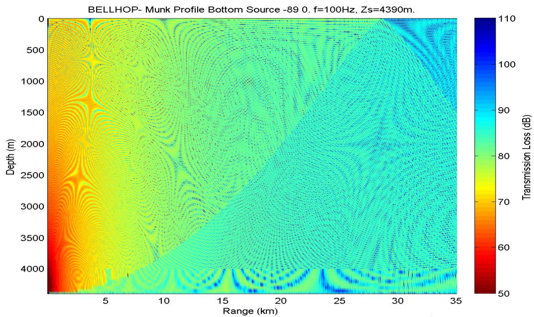
Figure 15. Constant bathymetry 100 Hz Transmission Loss; receiver at 4390 m.
