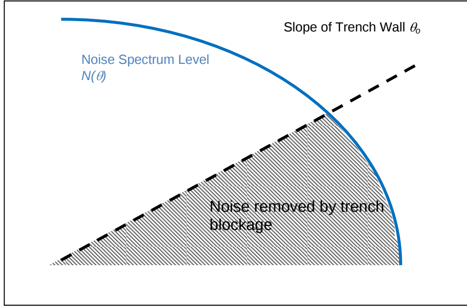
Figure 28. Graphical representation of the noise calculation showing the noise removed by the trench slope \theta_0 .
