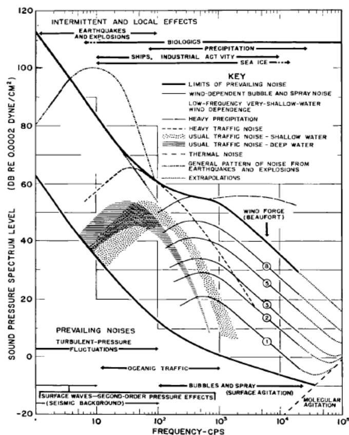
Figure 6. A composite of ambient noise spectra (from [13]).
