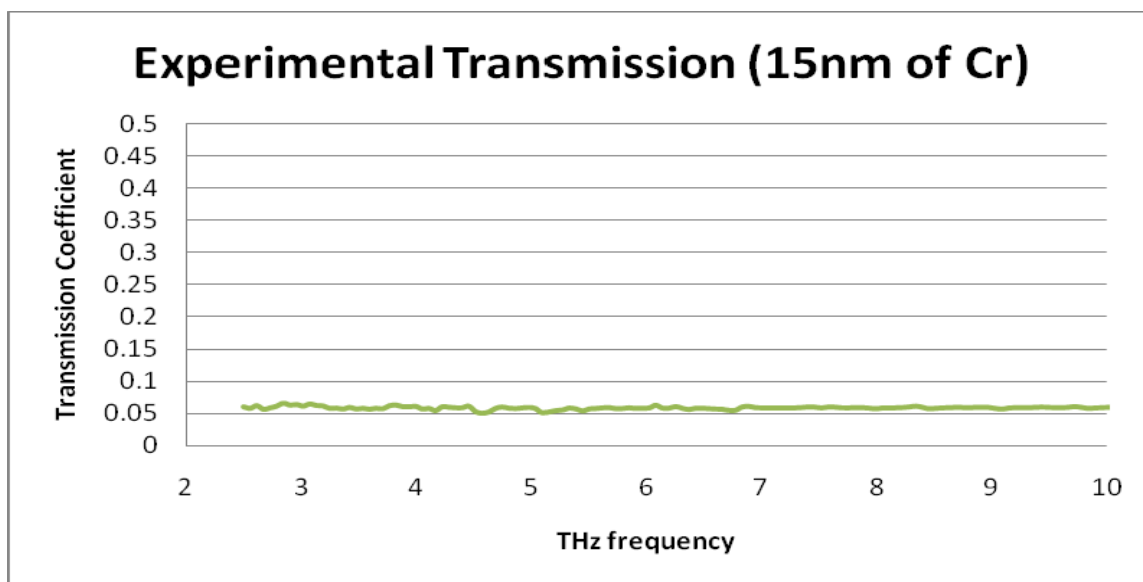
Figure 21. Experimental Transmission of the Multi-layer Stack of 15 nm of Cr as a Function of THz Frequency
