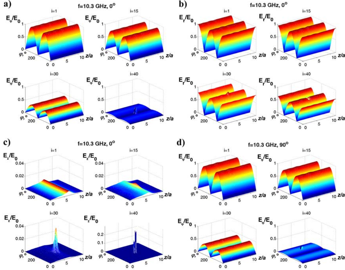
Fig. 18. Distributions of components of the electric field in the waveguide with the SE on the different surfaces \varphi 0z at f = 10.3 \text{ GHz} : E_\varphi at \varphi = 0^\circ (a) and \varphi = 90^\circ (d) for r = (i-1)\Delta r ; E_r at \varphi = 0^\circ (b) for r = (i-0.5)\Delta r ; E_z at \varphi = 0^\circ (c) for r = (i-0.5)\Delta r ; Calculation parameters: \Delta r = 0.025 , \Delta z = 0.05 , \Delta \varphi = 2.8^\circ , \Delta t = 4.50 \cdot 10^{-4} . Dimensions of the SE are h \times d \times l = 0.5 \times 2.9 \times 5 \text{ mm}^3 , \rho = 20 \text{ } \Omega \cdot \text{cm} , a = 10 \text{ mm} .
