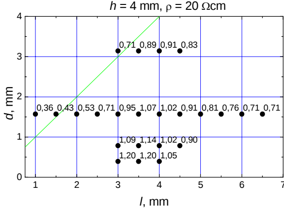
Fig. 21. The ratio \langle E_\phi \rangle(14.5)/\langle E_\phi \rangle(10.3) versus longitudinal and transverse dimensions of the SE for \rho = 20 \text{ } \Omega\text{cm} material and fixed height h = 4 \text{ mm} . The number near the point corresponds to the value of the ratio for the particular pair of d and l . The solid curve in the figure corresponds to d and l at which the DC resistance of the RS is 50 \text{ } \Omega , a = 10 \text{ mm} .
