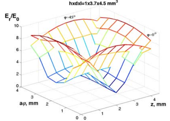
Fig. 8. Distributions in a \varphi = 0 plane of the component E_r in the obstacle at a resonance conditions: \varphi = 0^\circ , f = 11.0 GHz, \varphi = 45^\circ , f = 12.4 GHz. Dimensions of the obstacle are indicated in the figure.
