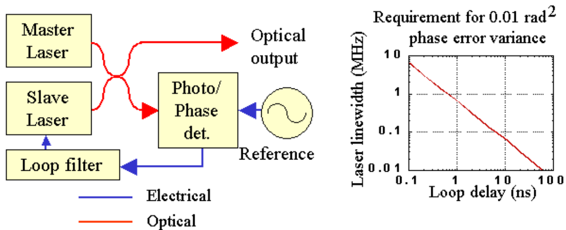
Figure 2: Optical phase lock loop.
