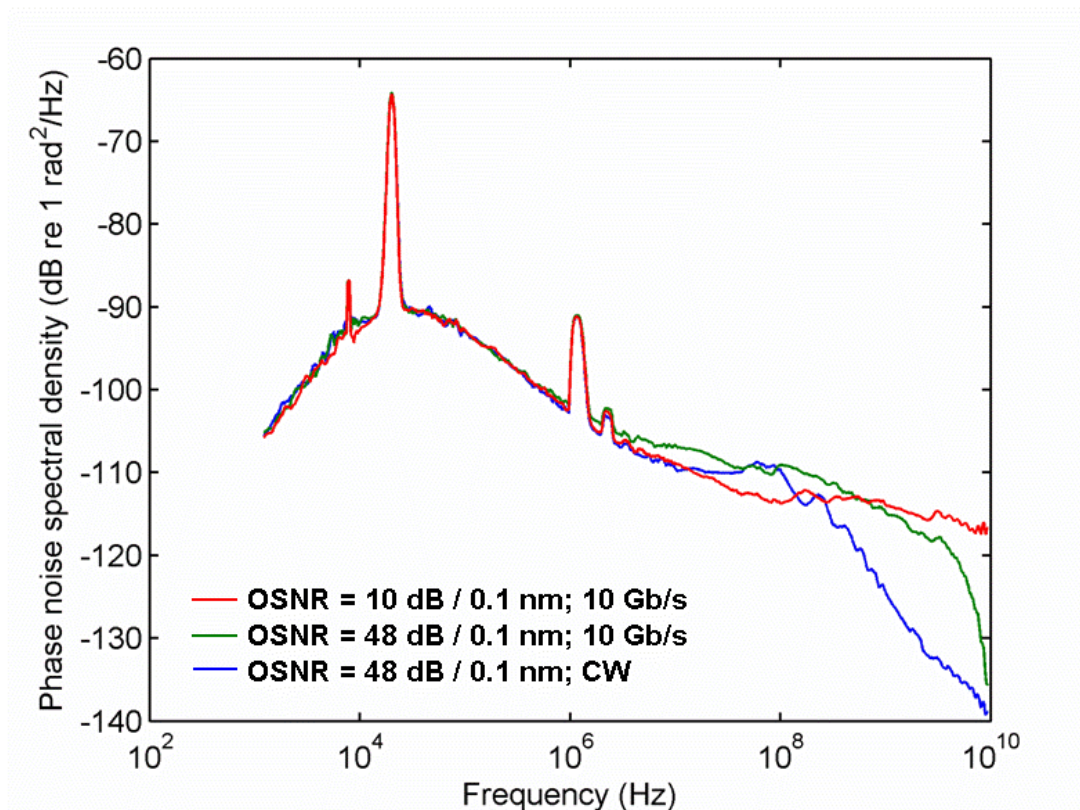
Figure 10: Phase noise spectrum with data modulated master signal.
