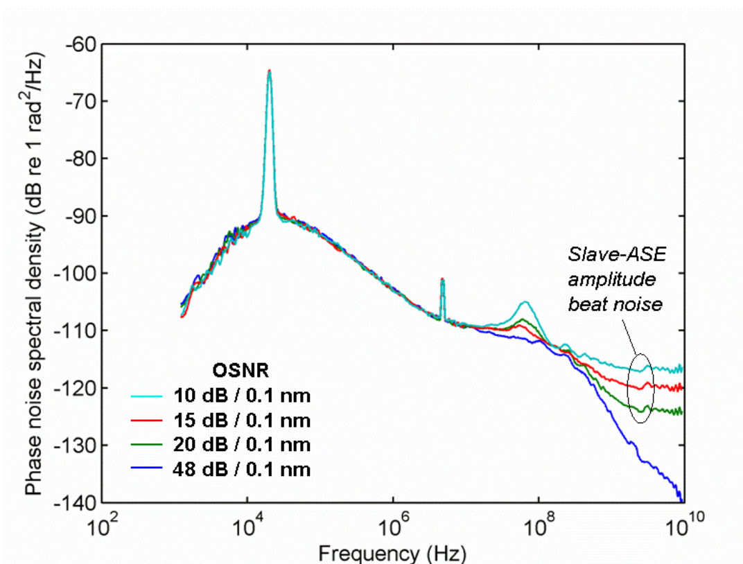
Figure 9: Phase noise spectra for noise-loaded CW master signal.
