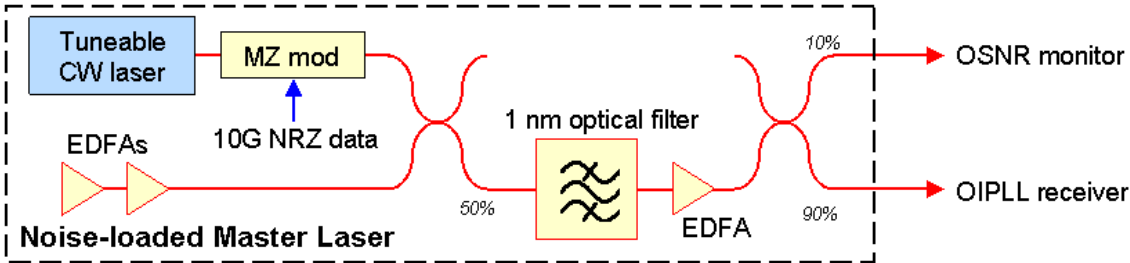
Figure 6: Noise-loaded transmitter.
