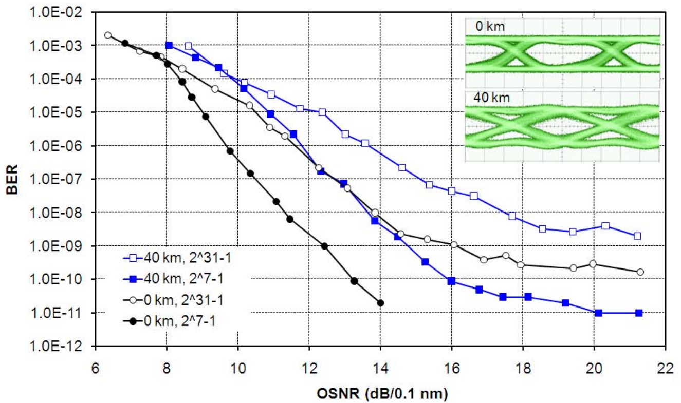
Figure 16: BER vs OSNR for coherent detection of ASK after 40 km of SSMF, compared to back-to-back performance (0 km). (The insets show the corresponding eyes, without noise loading.)
