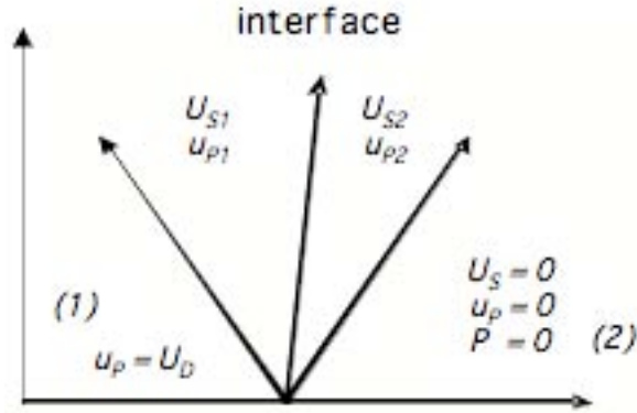
Figure 11. Impact details for impedance matching technique
