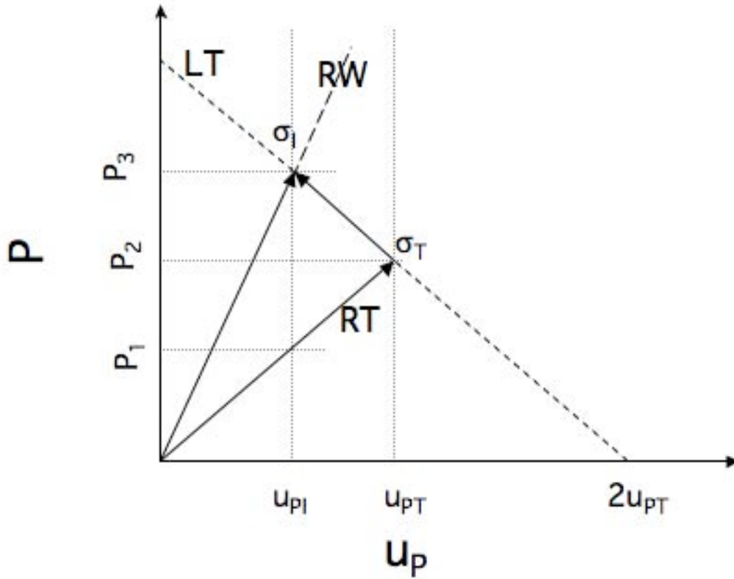
Figure 31. Cartoon P-up Diagram for Ceramic-Sapphire Interface
