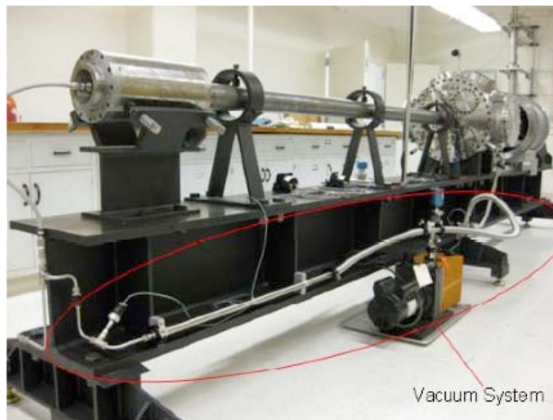
Figure 21. Vacuum System
