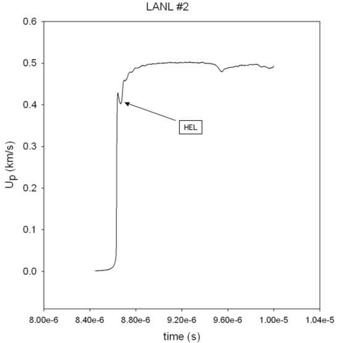
Figure 32. Wave profile from LANL shot 2
