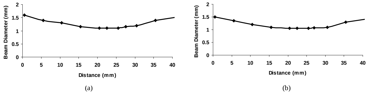
Figure 3. Beam diameter of Gaussian (a) and Flat-top (b) probes as a function of working distance. The spot diameters remain at approximately 1 mm diameter over a working distance of 15-30 mm.
