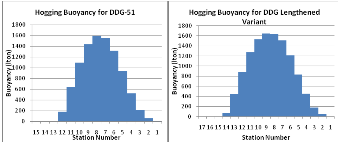
Figure 60. Hogging Buoyancy for Both Destroyers
