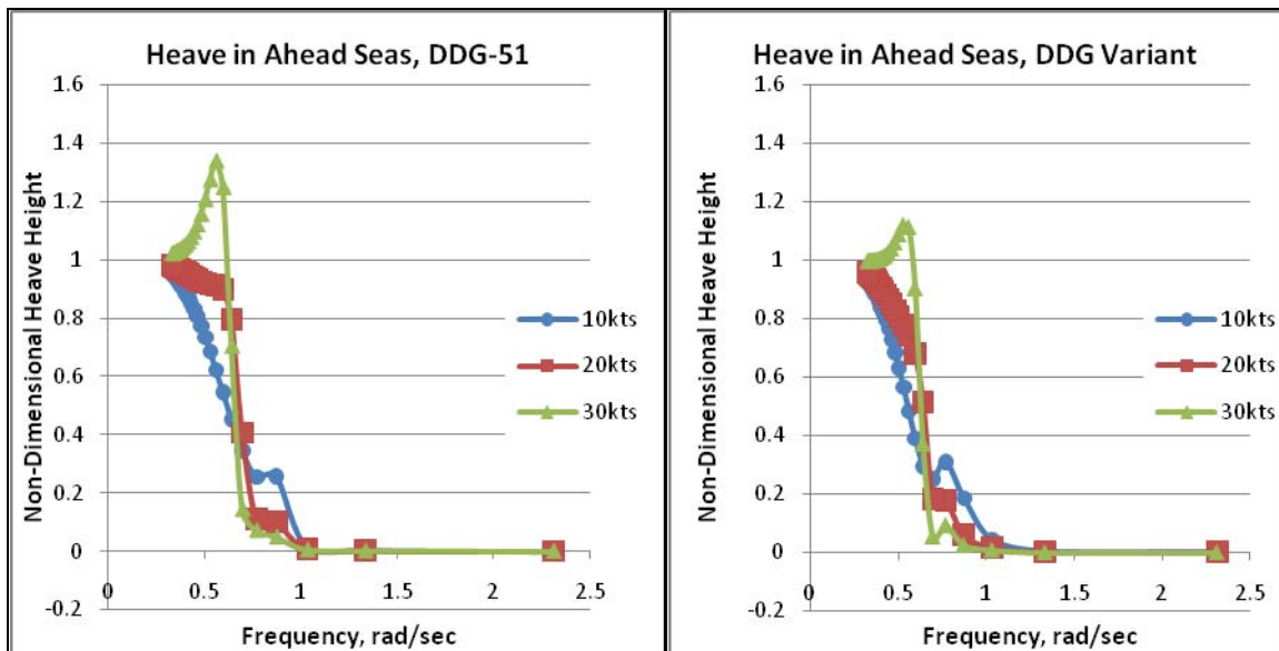
Figure 35. Heave Motion from Ahead Seas for Both Vessels
