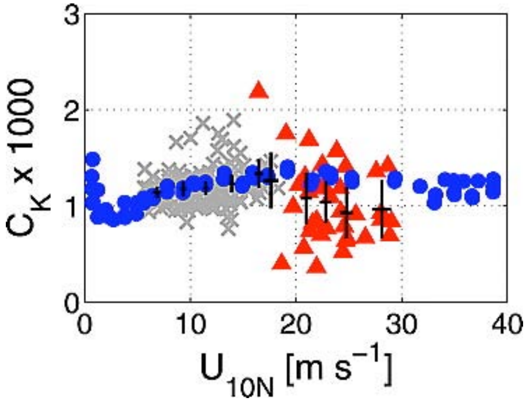
Figure 7. Wind speed dependence of C_K from Haus et al. (2010). ASIST laboratory results ( \bullet ) and CBLAST ( \blacktriangle ) measurements are shown with HEXOS results ( \times ). After binning observations by wind speed, the mean and 95% confidence intervals as determined from a t-distribution of the combined HEXOS and CBLAST field data are shown in black.
