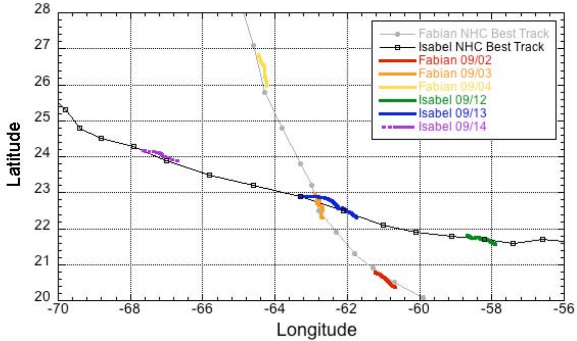
Figure 22. NHC best tracks (black and gray) and radar-derived tracks (color, see inset) used in this study for Hurricanes Fabian and Isabel.
