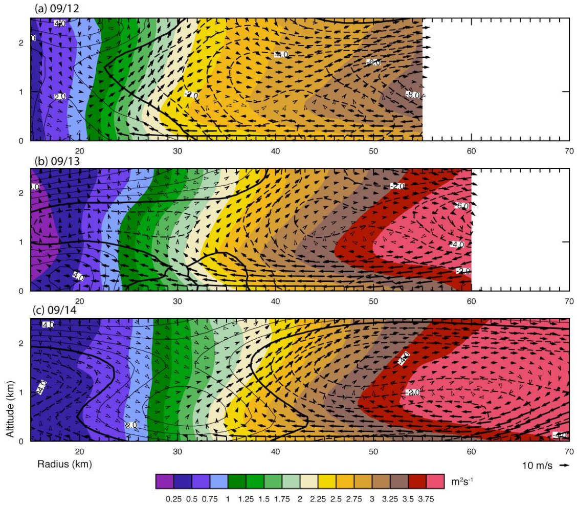
Figure 47. Isobaric axisymmetric angular momentum (color), total energy ( 350 \text{ kJ kg}^{-1} + 1 \text{ kJ kg}^{-1} contours), and secondary circulation (vectors) from 12–14 September.
