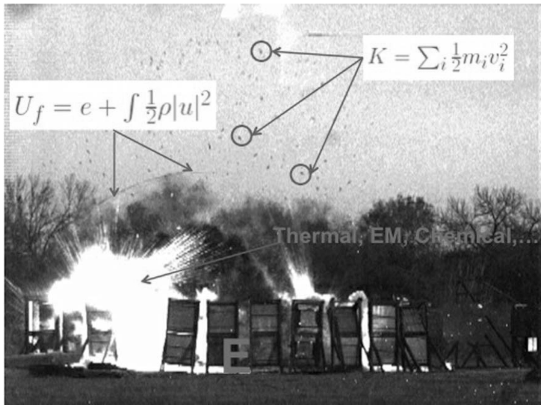
Fig. 1. The total energy conversion from detonation of an explosive charge resulting in kinetic energy of fragments ( K ), and a shock adiabat ( U_f ) together with excess thermal, chemical and electromagnetic pulses (EM). The shock wave and the associated blast wind are responsible for primary blast injury.
