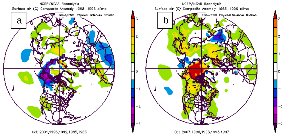
Figure 19. Composite anomalies of October surface air temperature (°C) for: (a) the five extreme high SIC years in the Beaufort Sea and (b) the five extreme low SIC years in the Beaufort Sea. Note the generally negative (positive) anomalies in the Beaufort Sea region in the high (low) SIC years.
