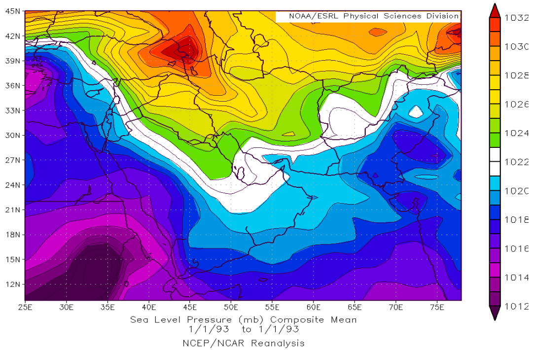
Figure 23. Sea Level Pressure, 1 January 1993.
