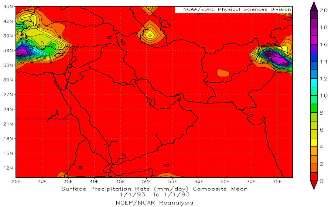
Figure 44. Surface Precipitation Rate, 1 January 1993.
