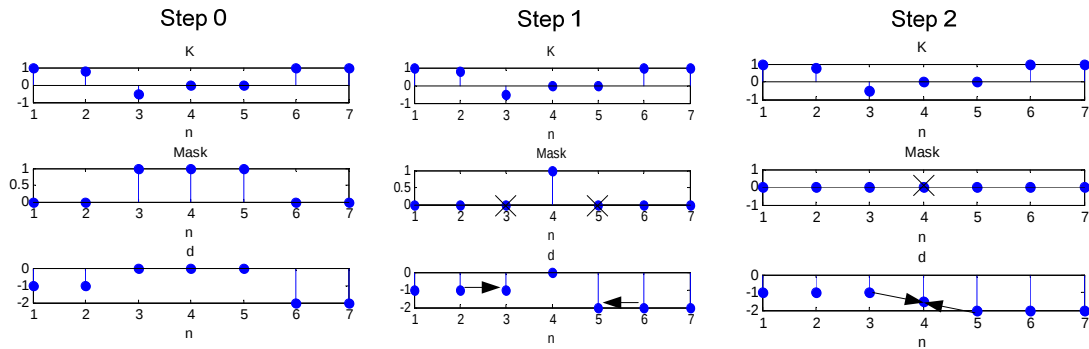
Figure 36. Illustration of Masked Averaged Hole Fill Algorithm.
