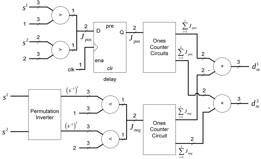
Figure 25. Distance Hardware.
