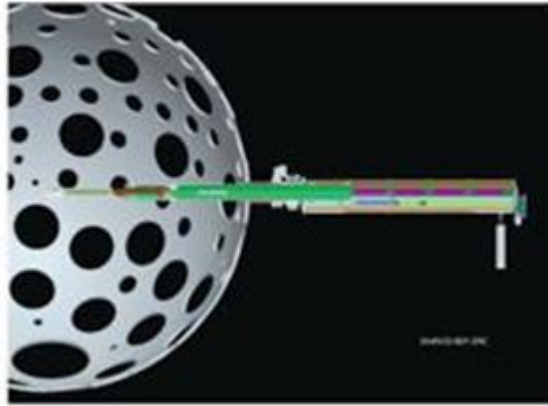
Figure 5. DIM and Chamber
